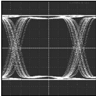
EQUALIZER OUTPUT EYE DIAGRAM AFTER 100FT OF BELDEN 9207 CABLE (DIFFERENTIAL, 2 7 -1 PRBS)
